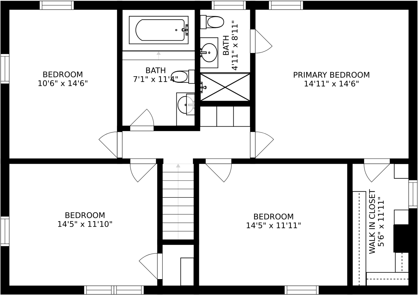
FLOOR 3
