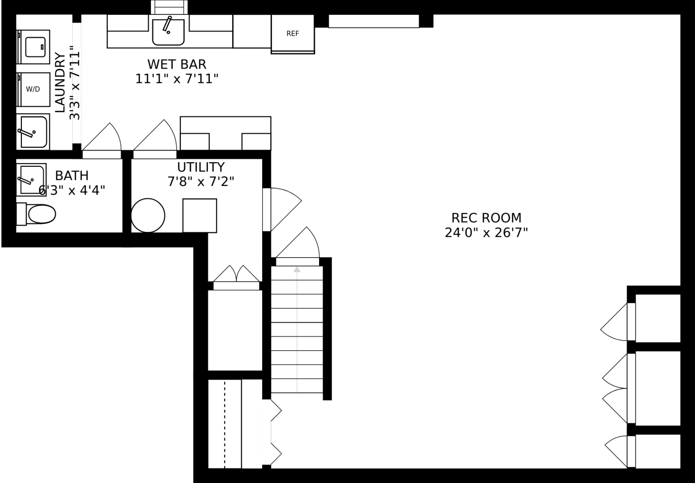
FLOOR 1
