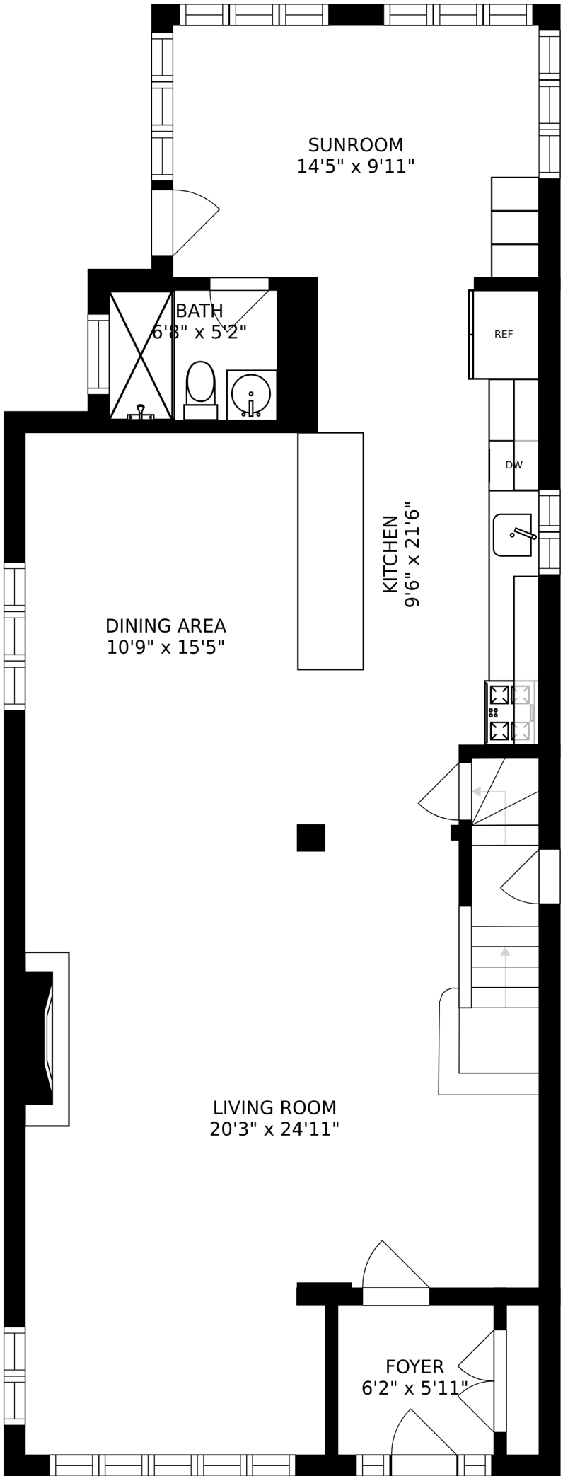
FLOOR 2
