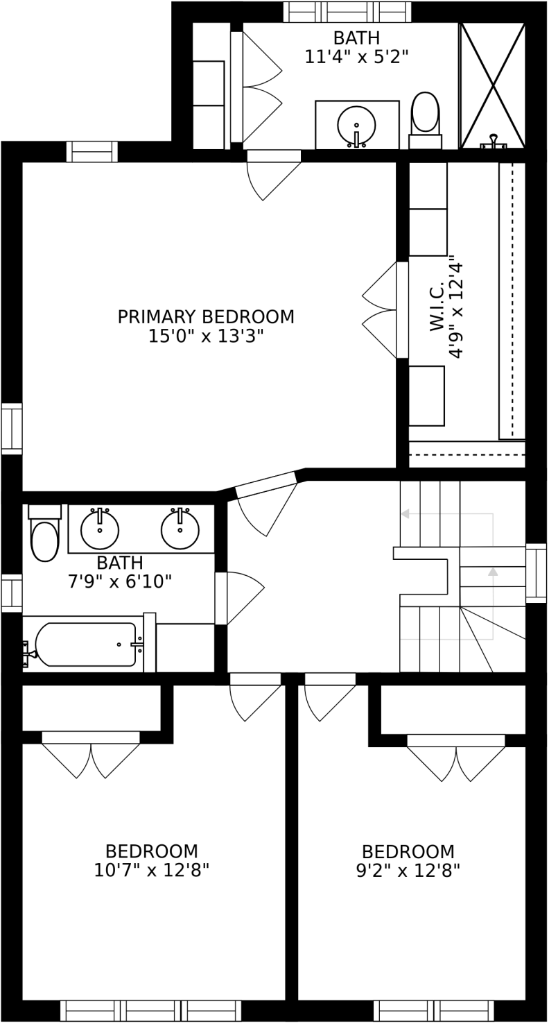
FLOOR 3
