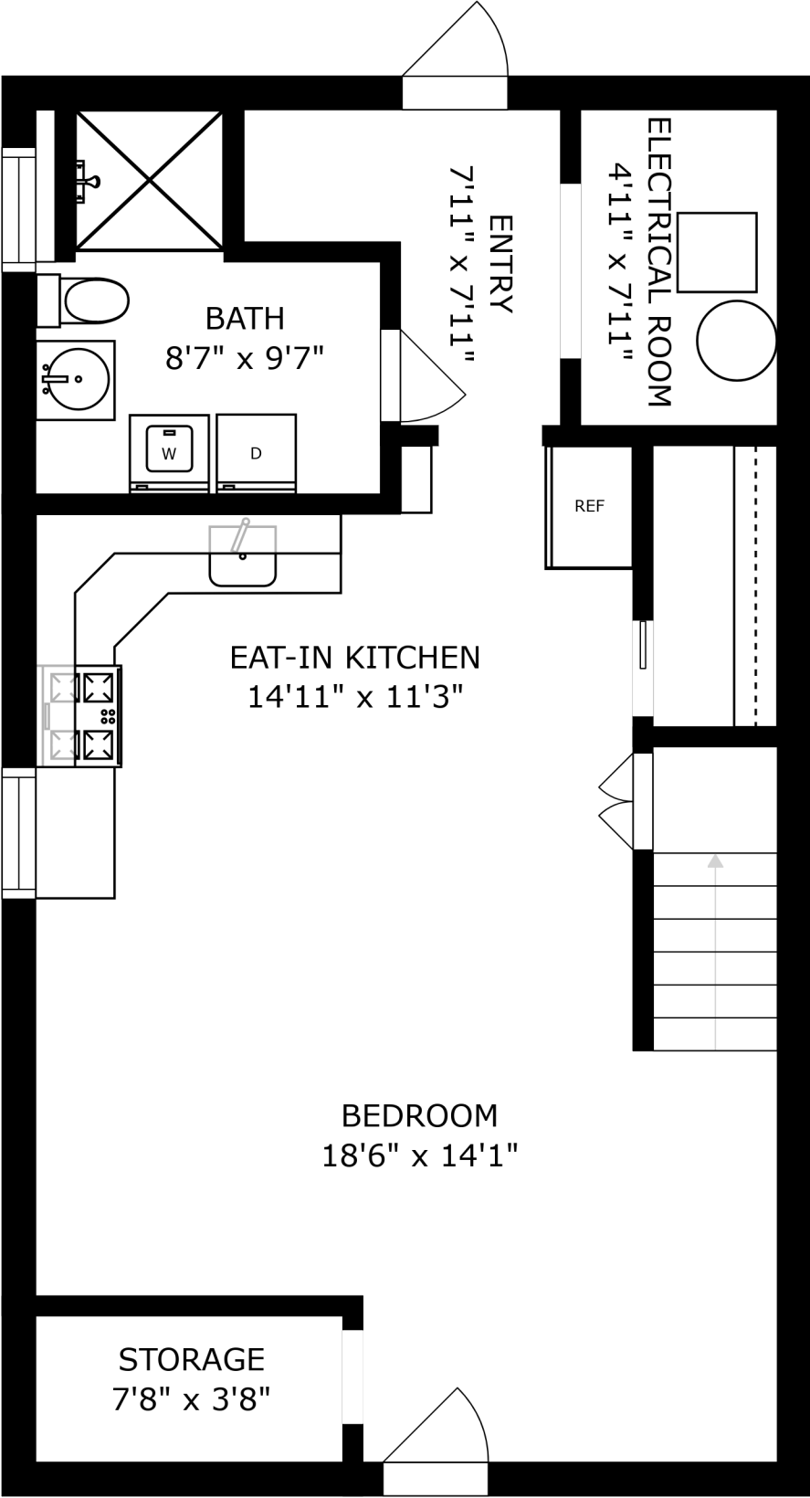
FLOOR 1
