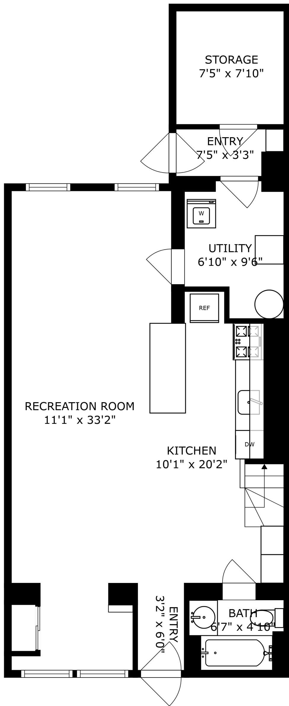
FLOOR 1
