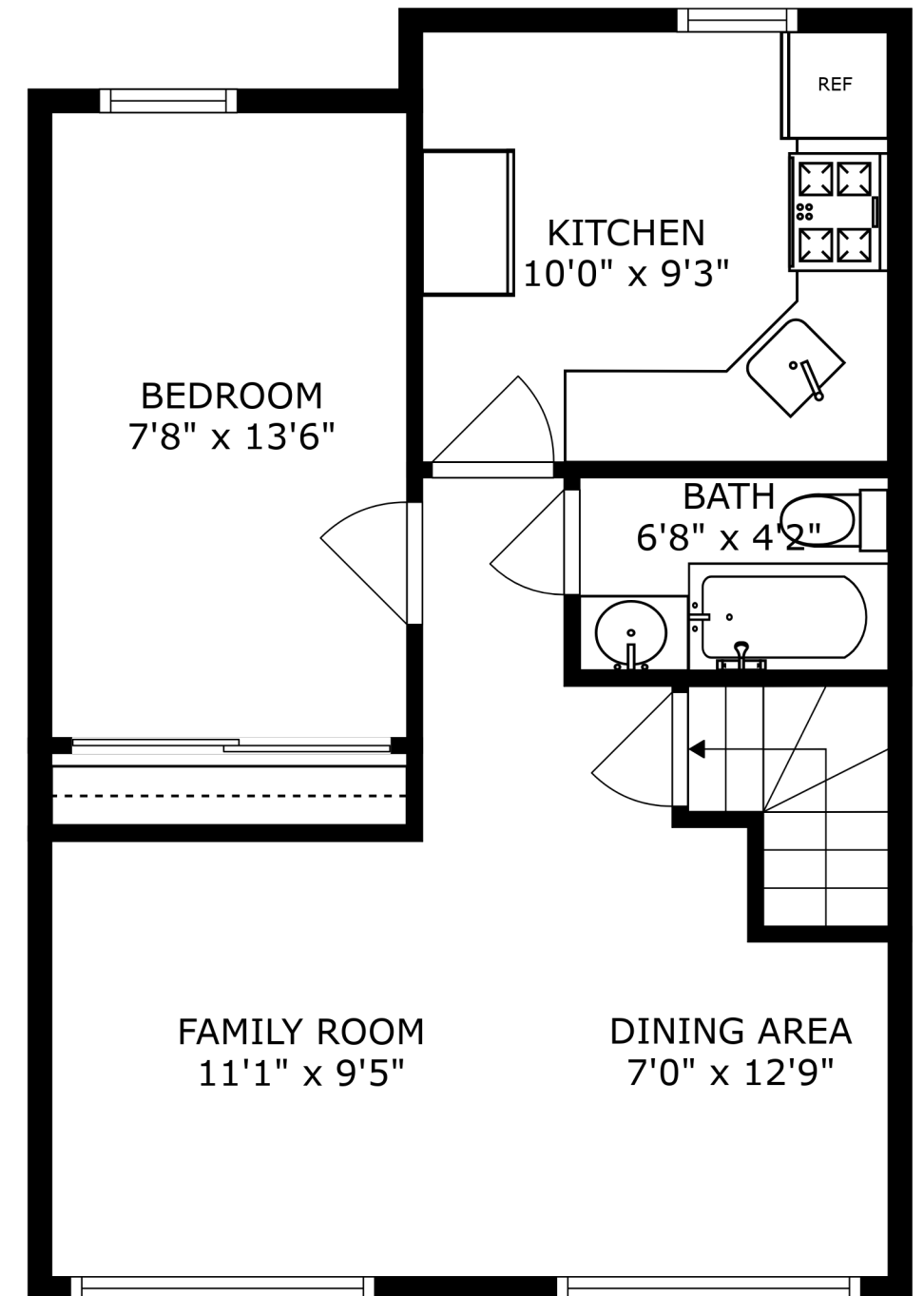
FLOOR 3
