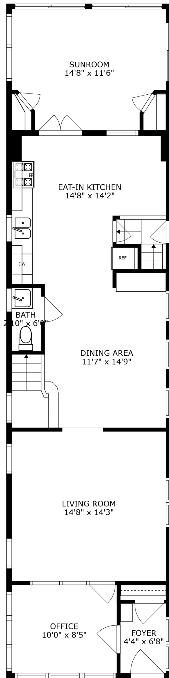
FLOOR 2
