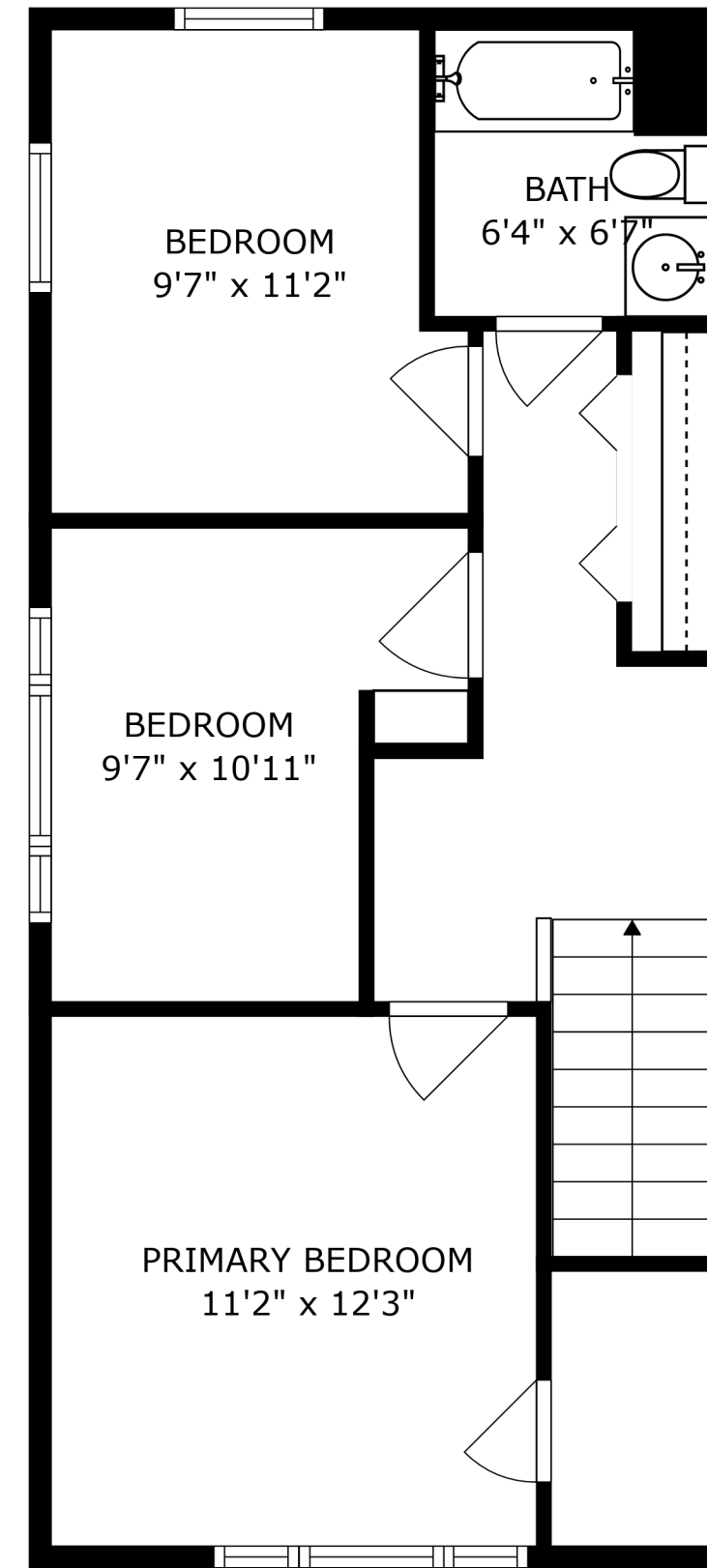
FLOOR 3
