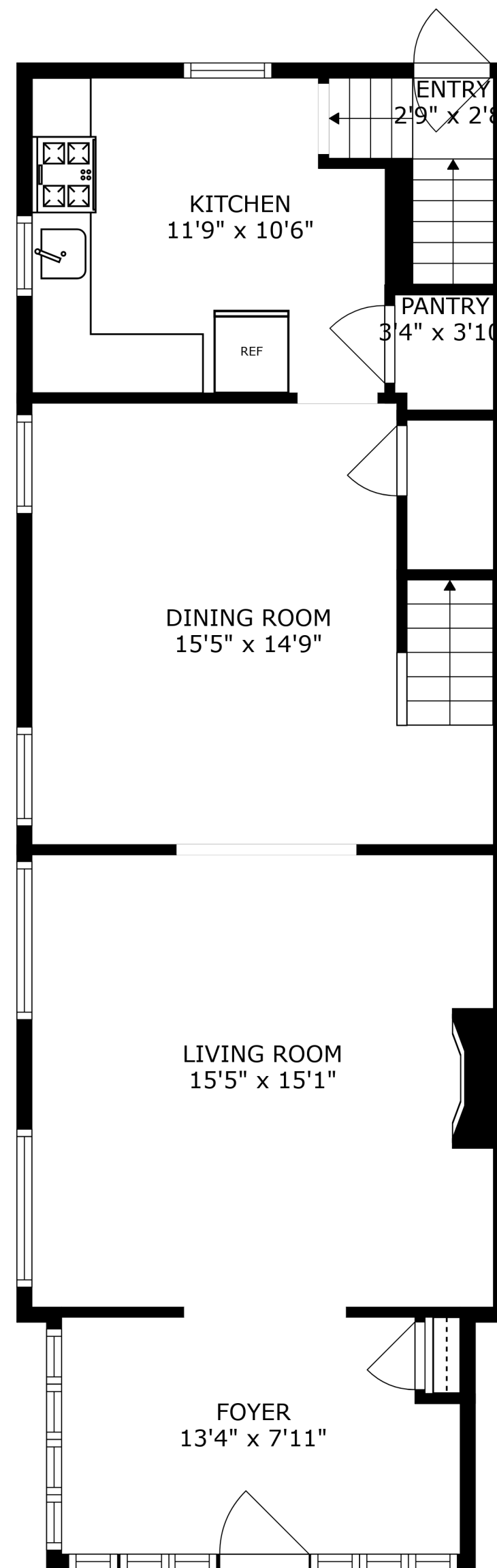
FLOOR 2
